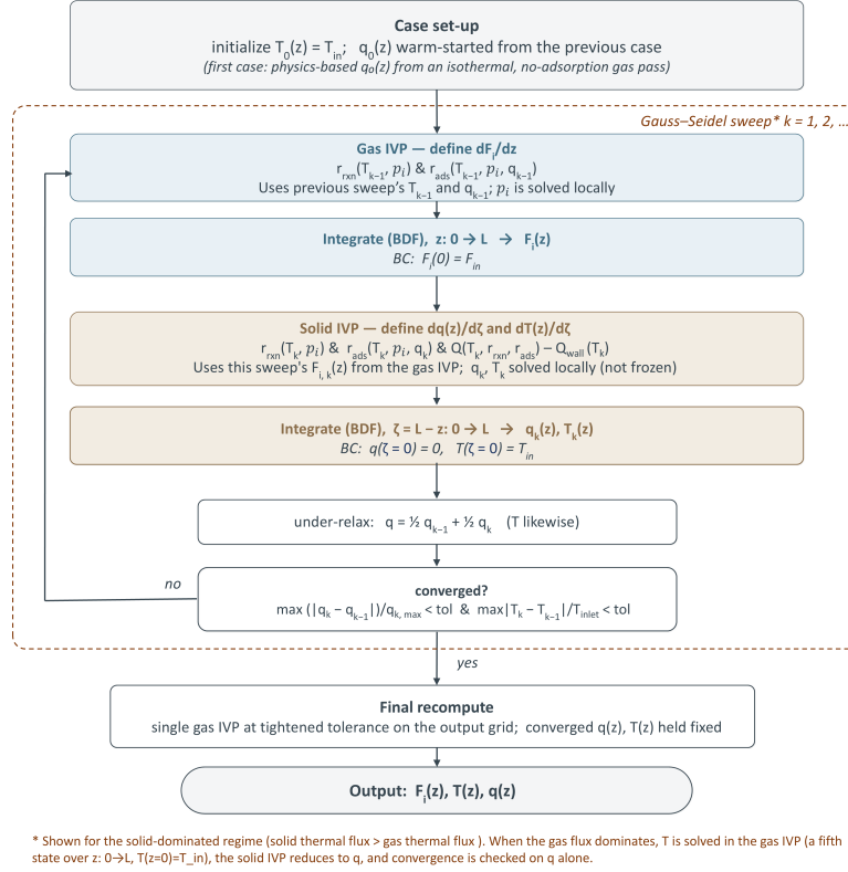
Figure 6.1: Solution algorithm for the steady-state, counter-current moving packed-bed (MPB) reactor model in molar-flux form.
