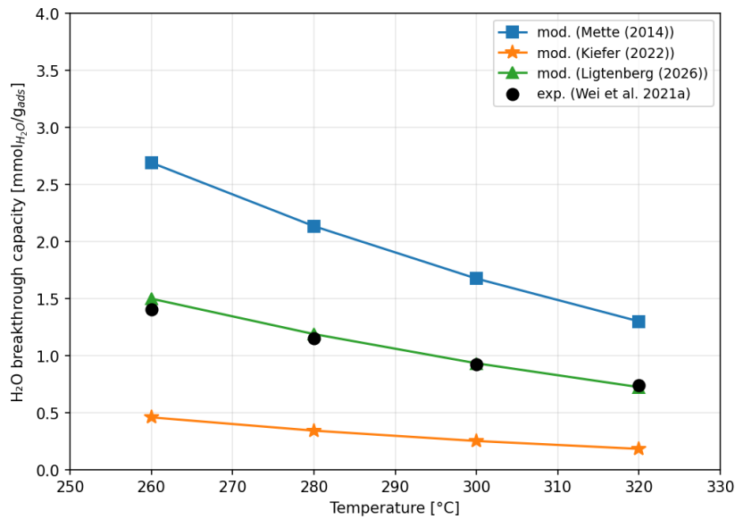
Figure 6.2: Water breakthrough capacity of zeolite 13X versus temperature, computed with a one-dimensional isothermal model assuming complete conversion, comparing three Dubinin–Astakhov parameter sets against the measurements of Wei. The set fitted in this work follows the data closely across the 280–300 °C operating window.
