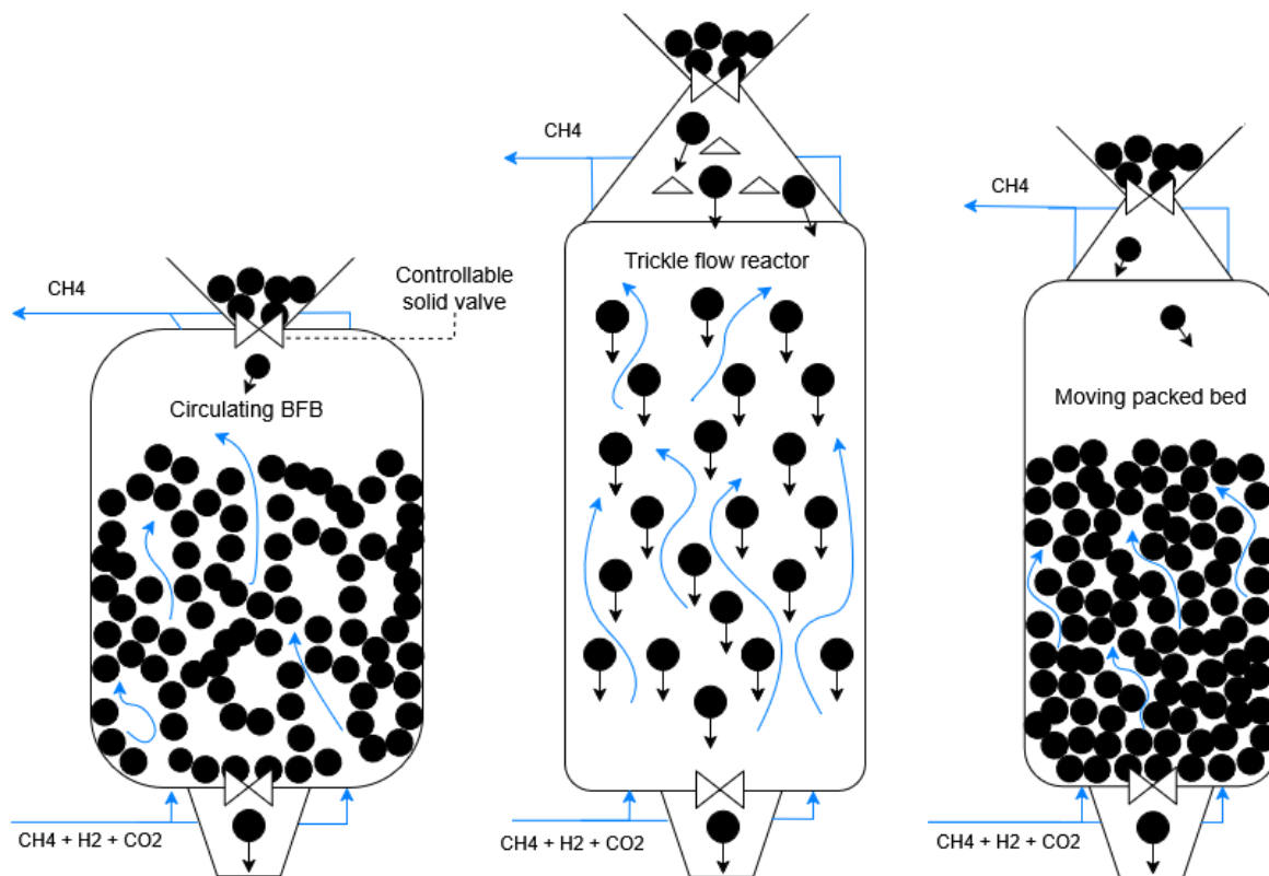
Figure 4.1: Schematic representation of the three continuous reactor configurations considered for sorption-enhanced methanation: circulating bubbling fluidised bed (left), trickle flow reactor (centre), and moving packed bed (right). Black spheres with arrows indicate the solid flow; blue arrows indicate gas flow. All configurations are shown as second-stage reactors receiving the partially converted outlet of a first-stage conventional methanation reactor, with \text{CH}_4 + \text{H}_2 + \text{CO}_2 as the inlet stream and \text{CH}_4 as the product stream at the top.
