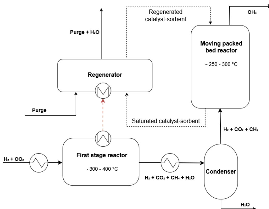
Figure 4.2: Block flow diagram of the two-stage sorption-enhanced methanation process. Dashed arrows indicate solid circulation; the red dashed arrow indicates heat transfer from the first stage to the regenerator.
