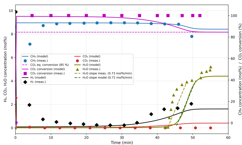
Figure 6.4: Model results validated against Wei (Fig. 5.10). Catalyst: 5%Ni2.5%Ce/13X; T = 240\text{ }^{\circ}\text{C} ; feed: 10 ml/min \text{H}_2 , 2.5 ml/min \text{CO}_2 , 81.5 ml/min \text{CH}_4 , 6 ml/min \text{N}_2 ; GHSV = 923\text{ ml g}_{\text{cat}}^{-1}\text{ h}^{-1} ; P = 1\text{ bar} . The experimental bed was regenerated with a 10% \text{H}_2 in \text{N}_2 mixture at 300\text{ }^{\circ}\text{C} and was therefore filled with this gas, rather than feed, at t = 0 ; the model initialises with feed concentrations and reacts immediately, which accounts for the discrepancy over the first 10 minutes. Thereafter the model overestimates the breakthrough time by approximately 5 minutes, consistent with batch-to-batch variation in the material's adsorption capacity. The model assumes 20 wt% active catalyst and is operated at 260\text{ }^{\circ}\text{C} .
